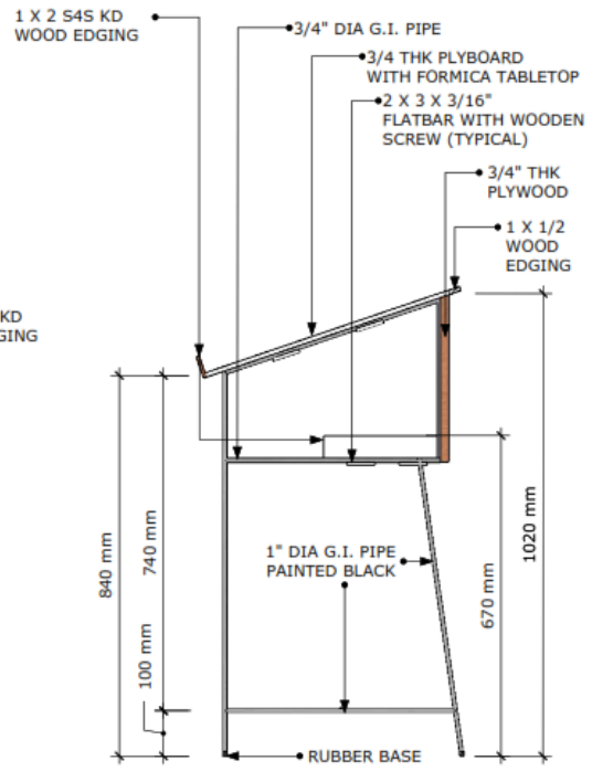
RIGHT SIDE VIEW SCALE 1:10M
