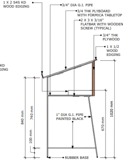
RIGHT SIDE VIEW SCALE 1:10M
