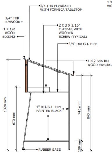
LEFT SIDE VIEW SCALE 1:10M
