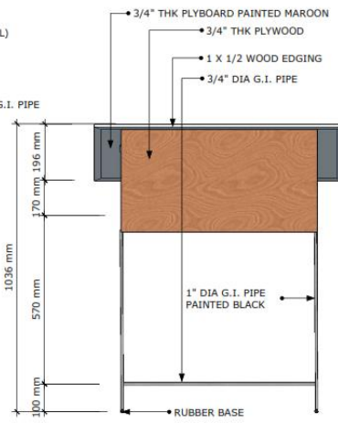
REAR VIEW SCALE 1:10M
