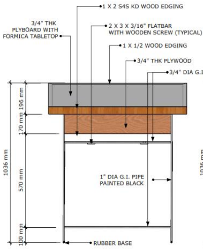
FRONT VIEW SCALE 1:10M
