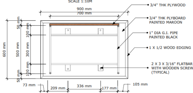
BOTTOM VIEW SCALE 1:10M
