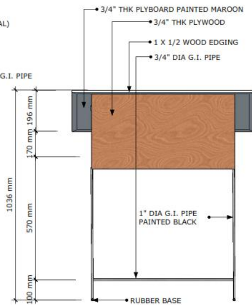
REAR VIEW SCALE 1:10M
