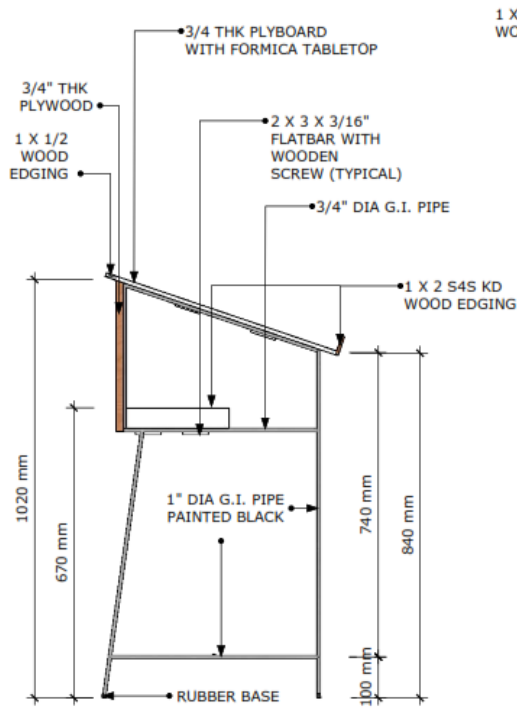
LEFT SIDE VIEW SCALE 1:10M
